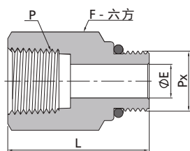
NPT 阴螺纹转 SAE/MS 阳螺纹
