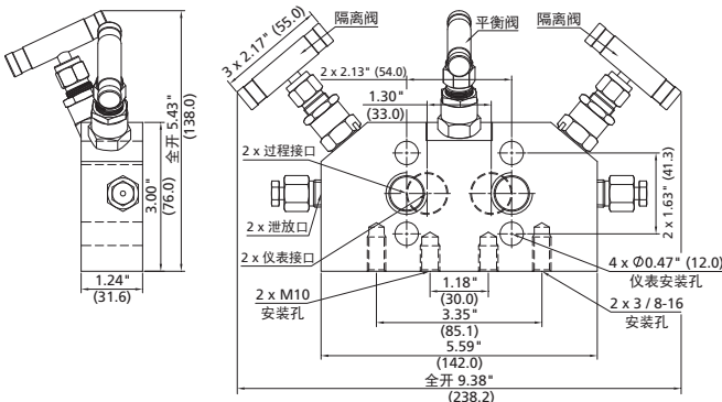
3D□□-FNS8-C-T
